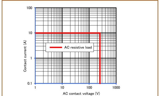
DLS1U (0.53W)
